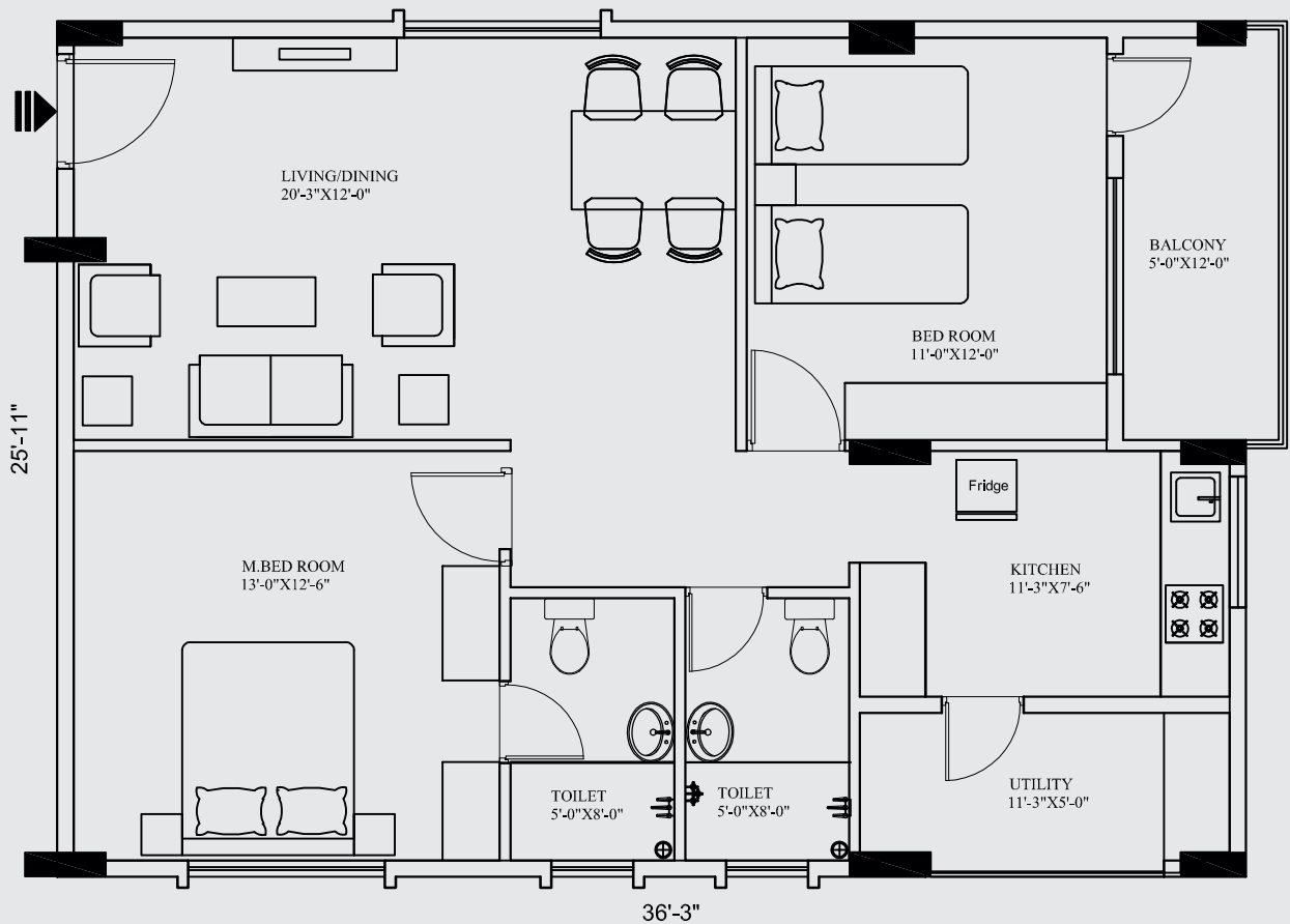
THIRD TO SEVENTH FLOOR
