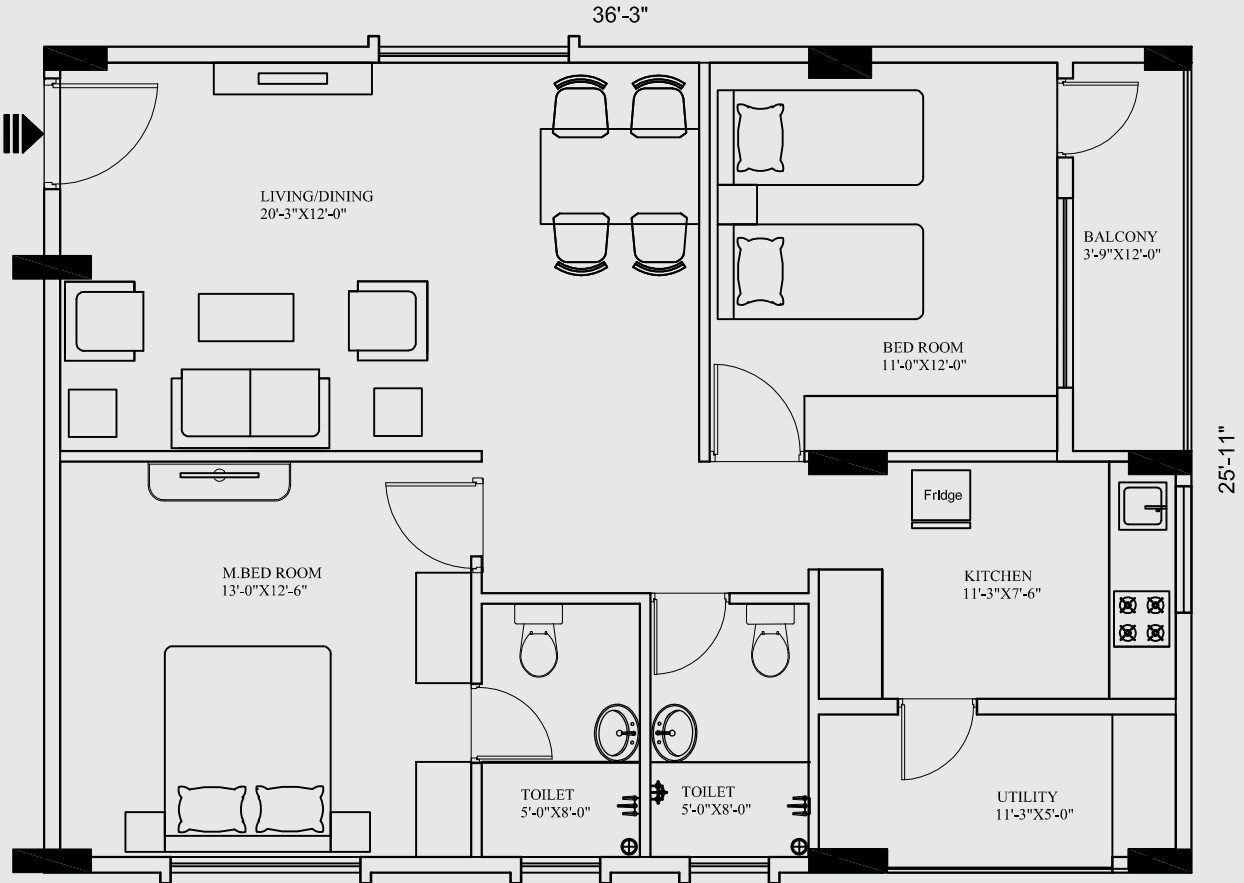
FIRST & SECOND FLOOR
